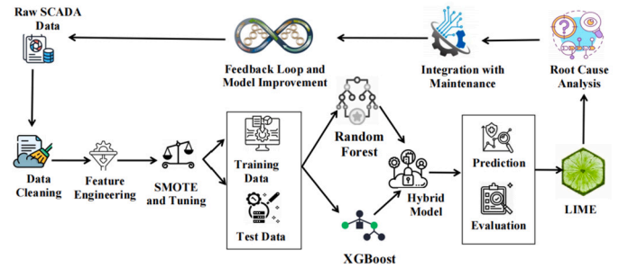
Fig. 3. Proposed Hybrid Model Architecture.
