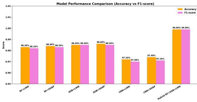
Fig. 19. Comparison with other XAI methods.
