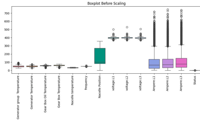
Fig. 7. Before Scaling.
