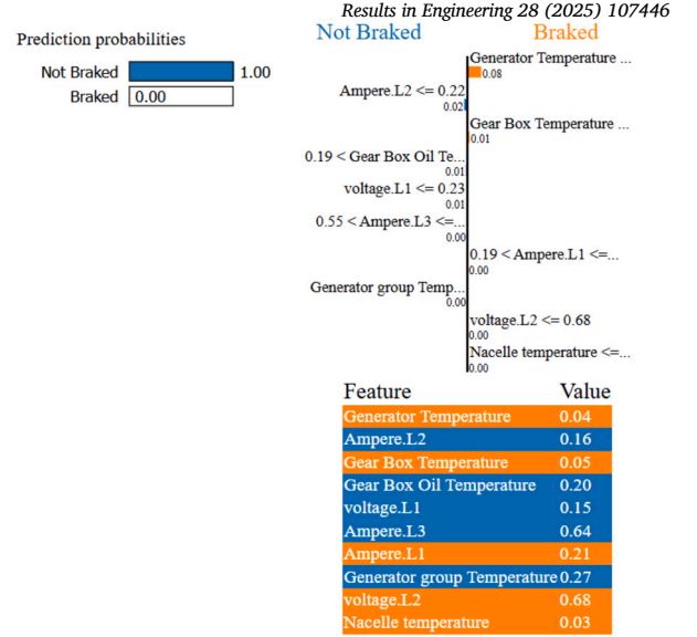
Fig. 12. LIME-based Explanation of Hybrid RF + XGBoost Model Prediction.
