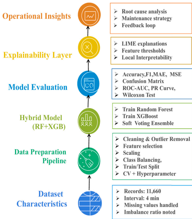
Fig. 4. Pipeline Diagram.
