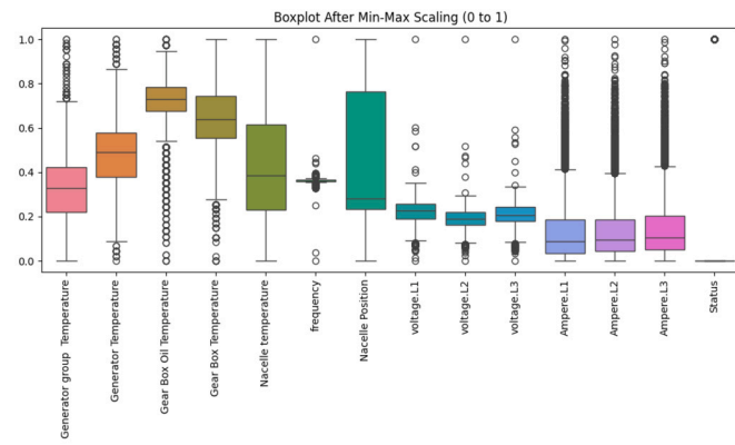
Fig. 8. After Scaling.
