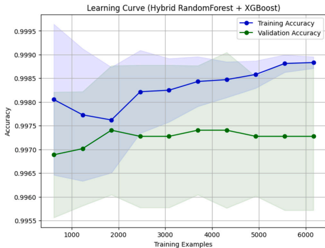
Fig. 18. Learning Curve.
