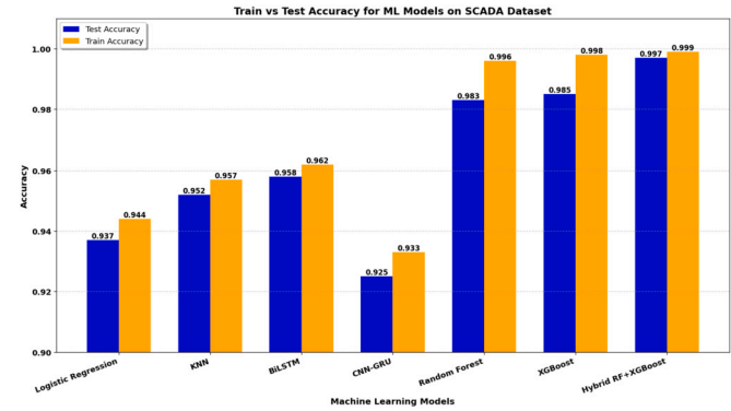
Fig. 14. Accuracy Comparison of Machine Learning Models.
