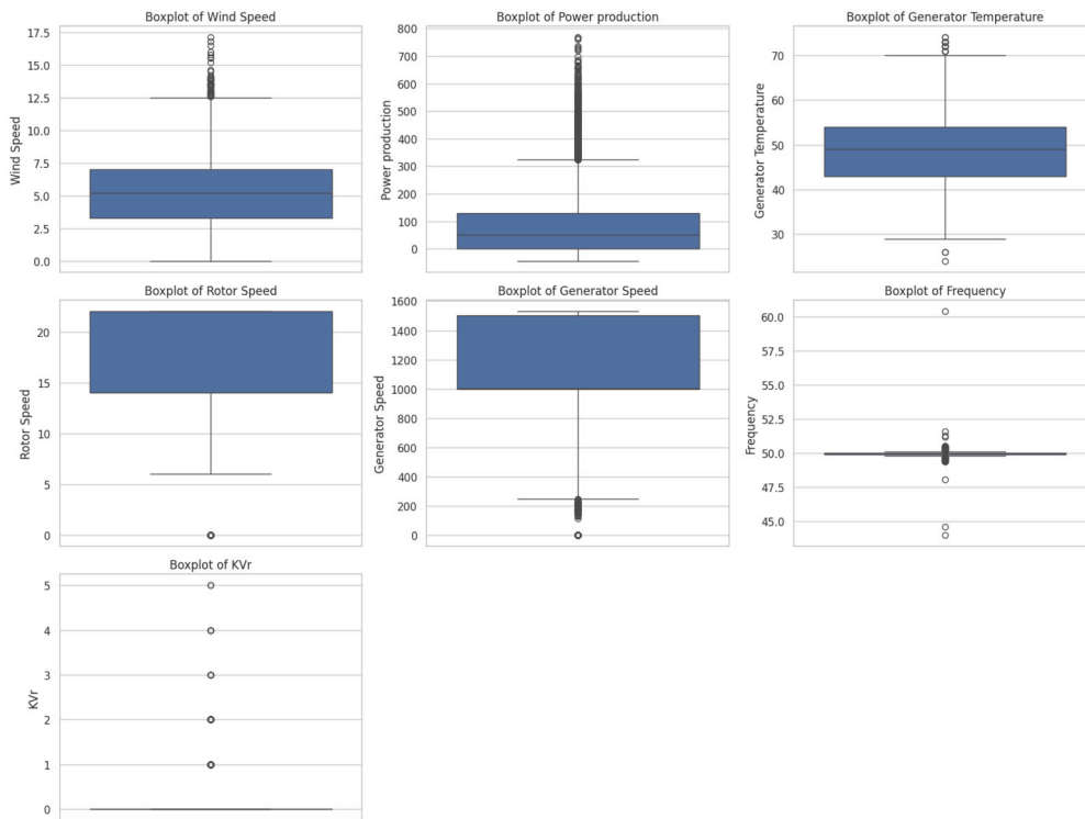
Fig. 6. Boxplot Analysis of SCADA Dataset Features.
