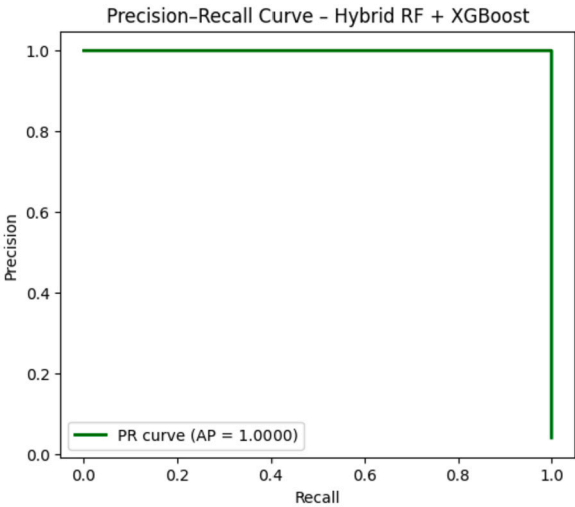
Fig. 16. Precision-Recall Curve.
